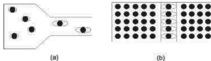
Fig. 10: Schematic representation of (a) micro homogeneous (b) craze-like deformation [68]
