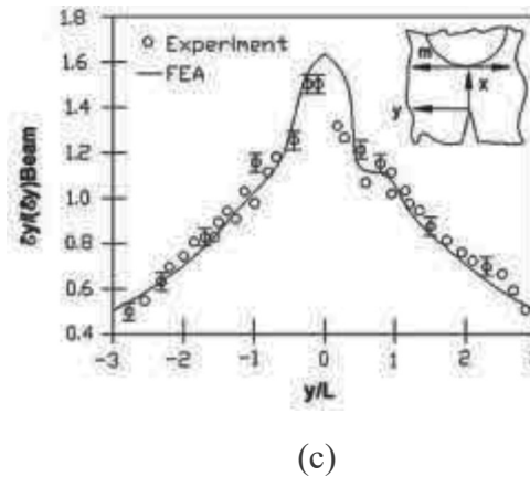
Fig. 6: Strain field evolution along (a) without inclusion (b) pre-debonding (with inclusion) and (c) post-debonding (with inclusion) stages [40,41].
