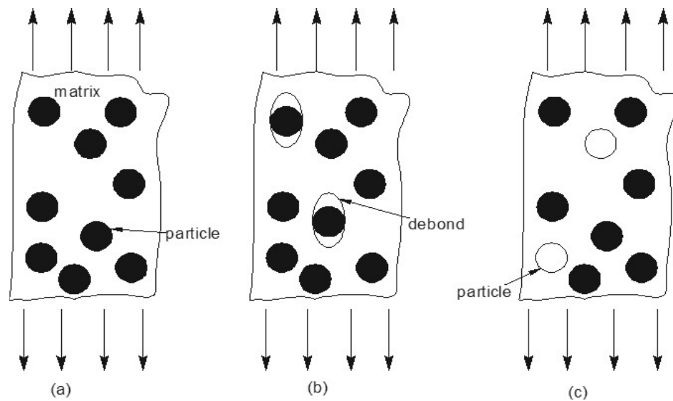
Fig. 9: Representation of particulate composites subjected to uniaxial tension: (a) undamaged (b) damaged by debonding at the apex (c) damaged by cavity formation [67].
