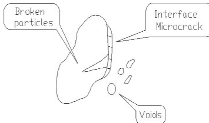
Fig. 1: Schematic diagram of different damage mechanisms in particle reinforced composites: particle breakage, interface debonding, and void growth in the matrix [11].
