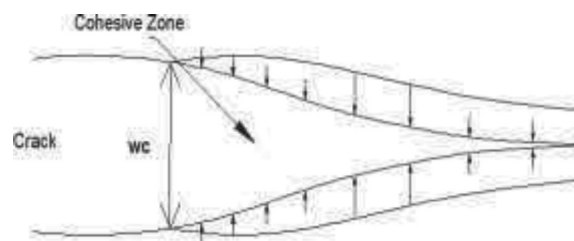
Fig. 4: Cohesive zone in mode I fracture [43]
