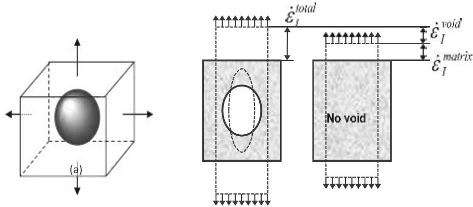
Fig. 3: Typical cell model, (a) with a central void, (b) additive behavior of strain rate due to voiding and strain rate in the matrix [24,26].
