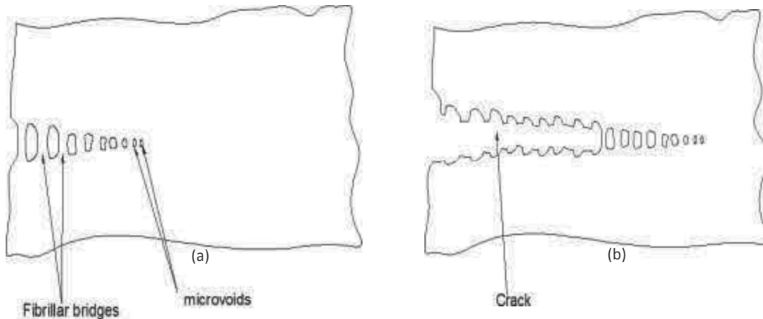
Fig. 2: Schematic drawings of (a) a craze showing microvoids and fibrillar bridges and (b) a craze followed by a crack [4]
