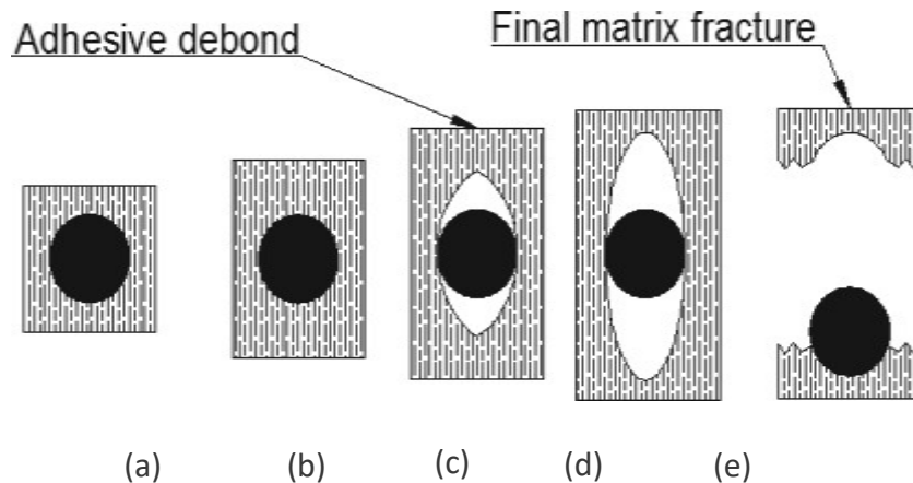
Fig. 8: Schematic of microdamage evolution in PMMA/ATH with a weak interfacial bond; (a) unloaded stage, (b) elastic deformation of matrix, (c) adhesive debonding, (d) debonding of matrix from filler and (e) fracture of matrix [63].
