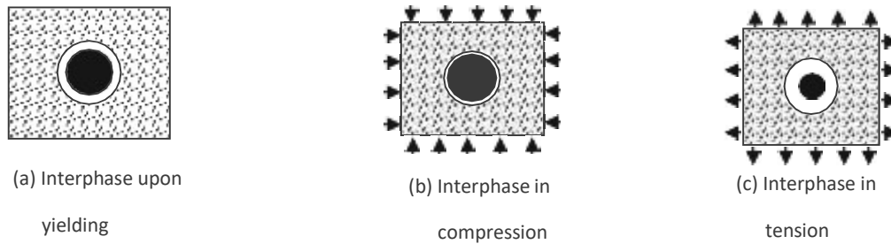
Fig.12: The influence of the second phase particle on void damage [25].
